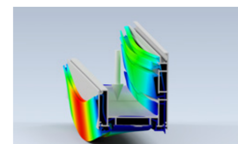
Stress test simulation on the gutter profile.
